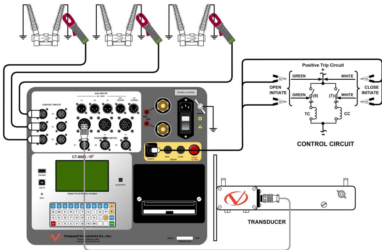
Figure 9. Typical Connections for Optional Dual Ground Testing Mode
